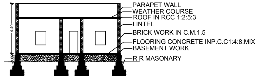
SECTION
