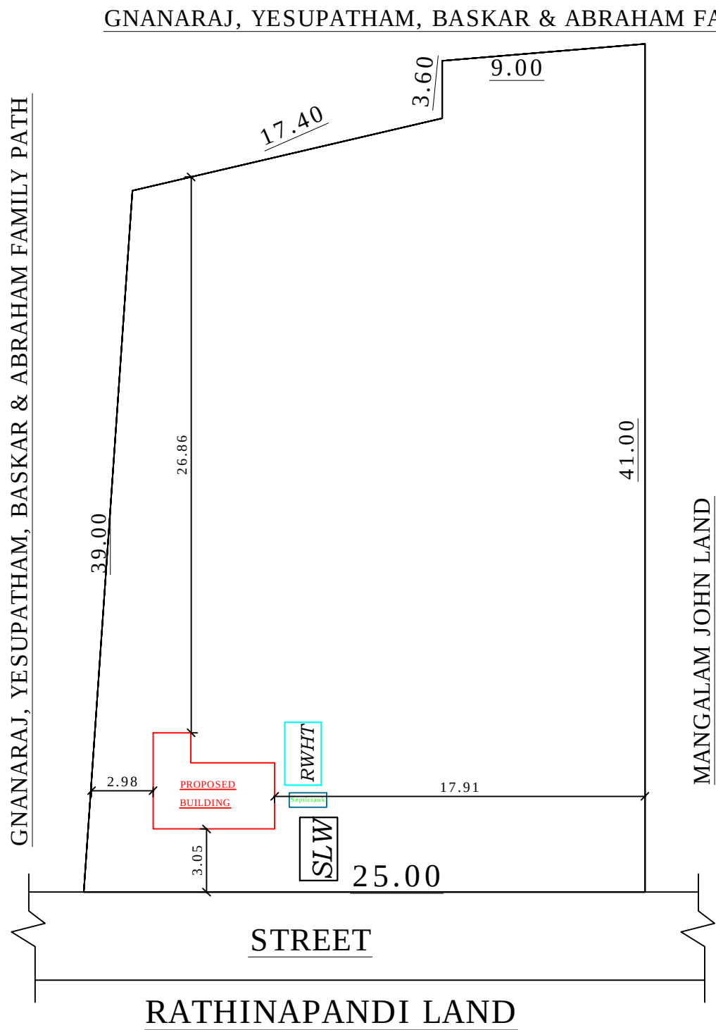
SITE PLAN
