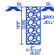
PERCOLATION PIT
