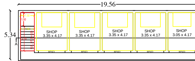
PRO. FIRST FLOOR PLAN
