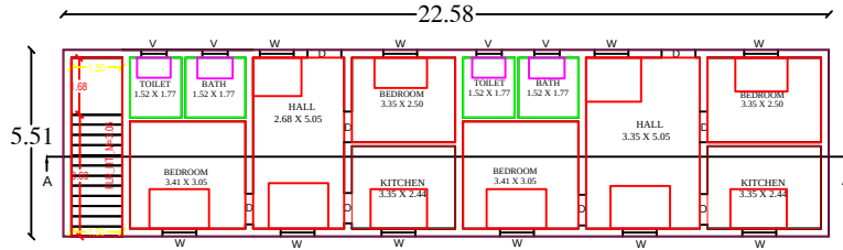
PRO. GROUND FLOOR PLAN
