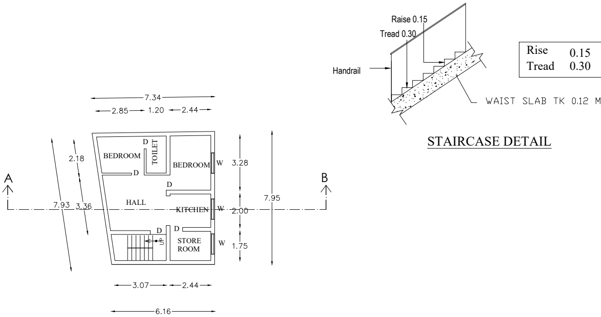
PRO GROUND FLOOR PLAN
