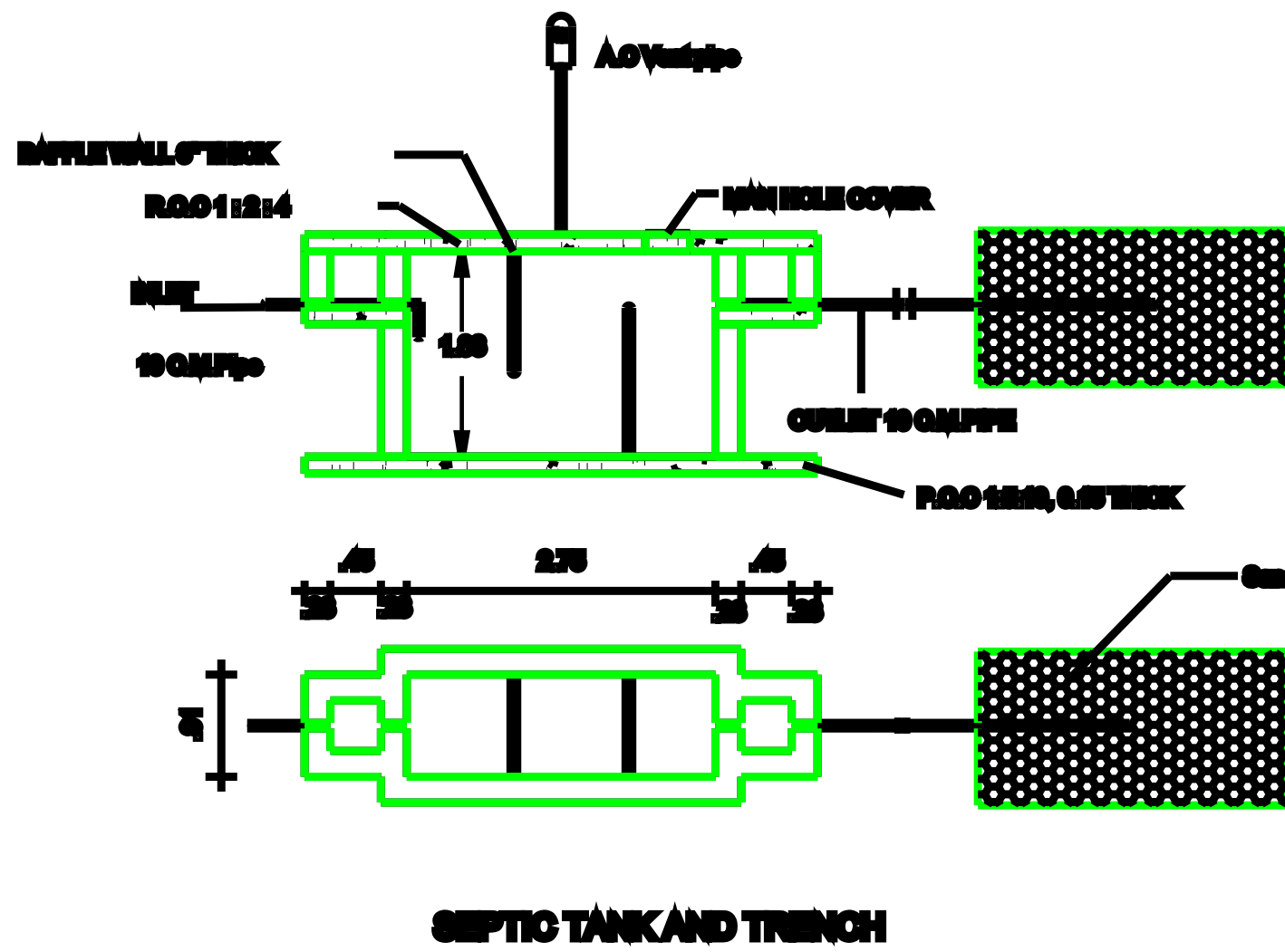
SEPTIC TANK AND TRENCH
