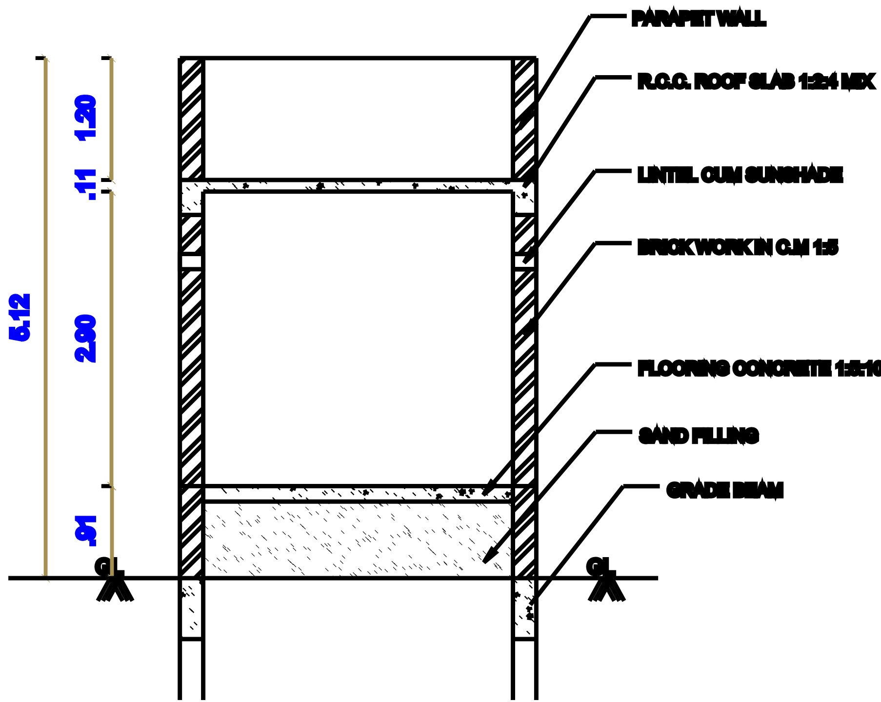
SECTION-AA
