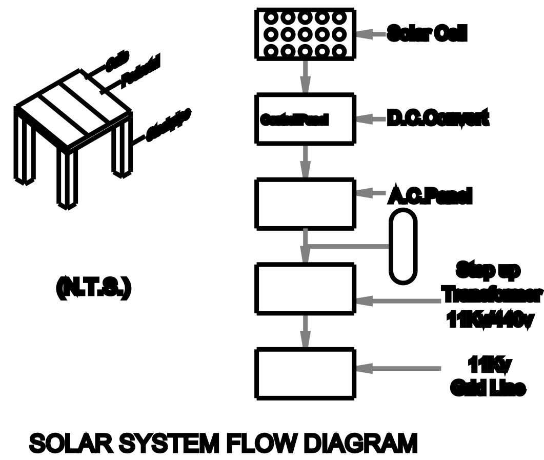
SOLAR SYSTEM FLOW DIAGRAM
