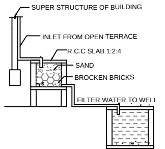
DETAILS OF FILTER BED & WELL
