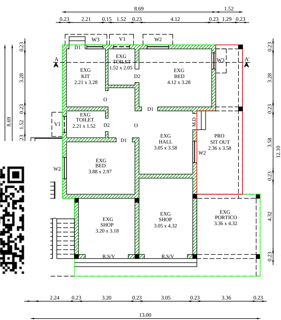
EXG & PRO.GROUND FLOOR PLAN
