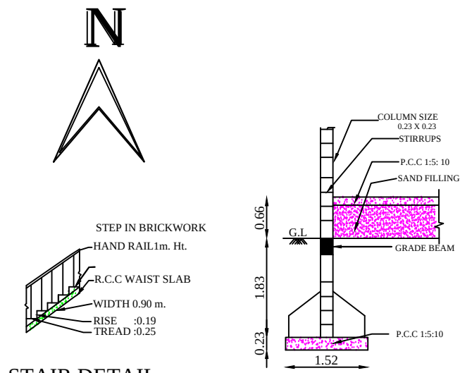
COLUMN DETAILS
