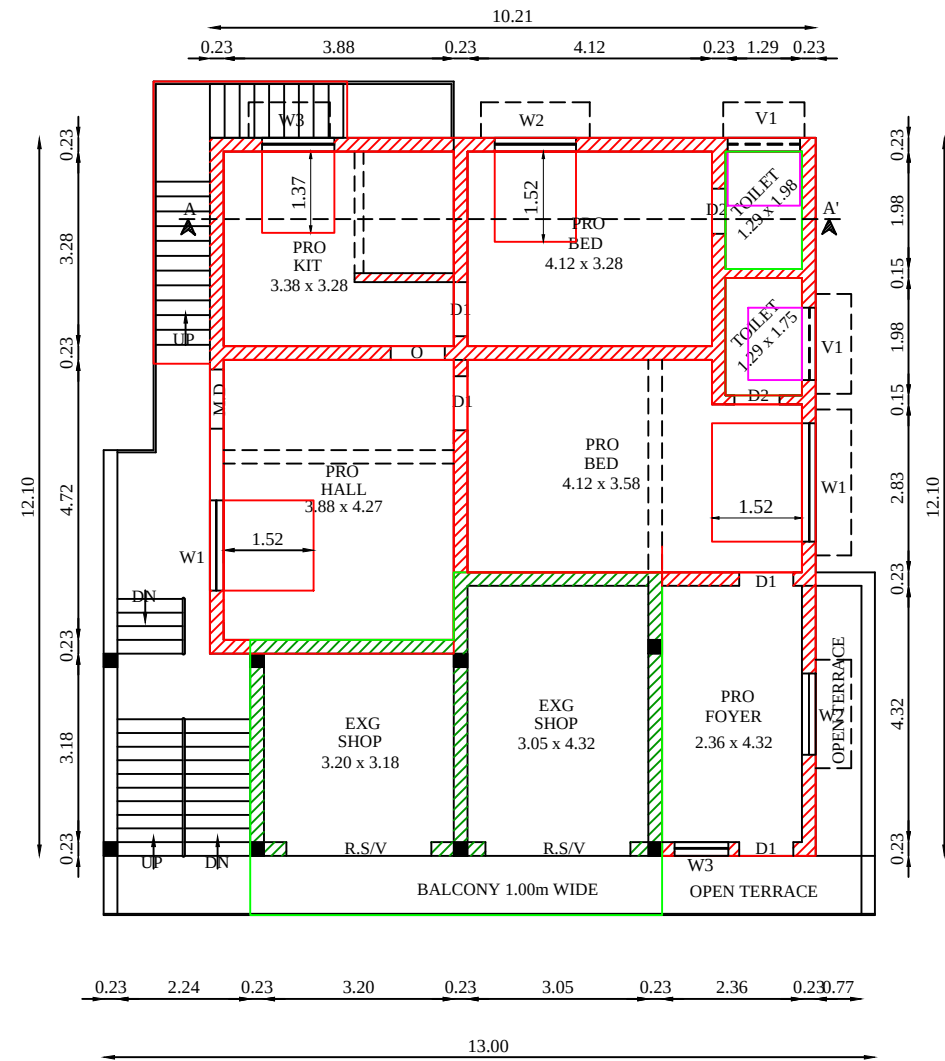
EXG & PRO.FIRST FLOOR PLAN
