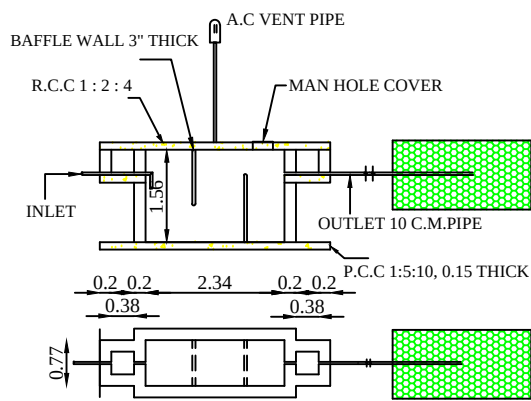
SEPTIC TANK AND DETAILS
