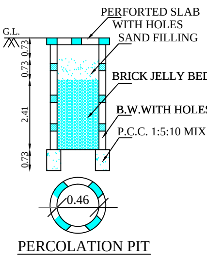
PERCOLATION PIT
