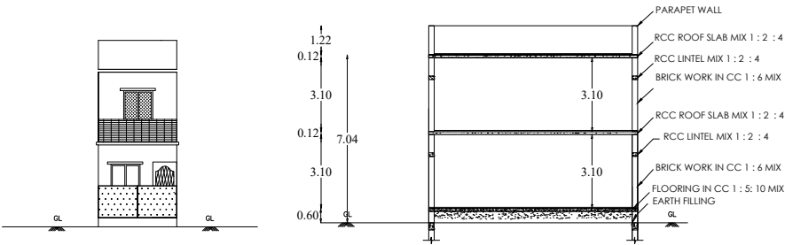
SECTION ON AB & ( HALF ELEVATION)
