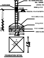
FOUNDATION DETAILS
