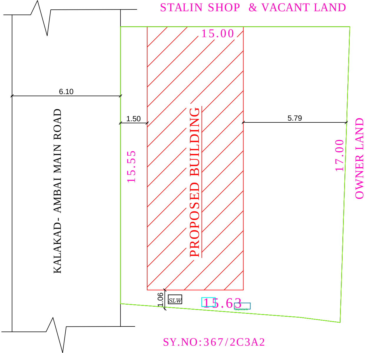
SITE PLAN
