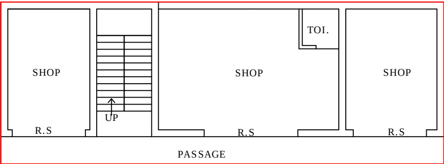
FIRST FLOOR PLAN (PROPOSED)
