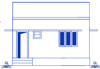
FRONT ELEVATION
