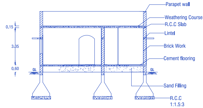
CROSS SECTION ON 'AB'
