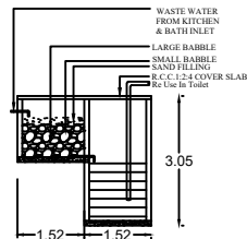
RECYCLING OF WASTE WATER FROM KITCHEN & BATHROOM
