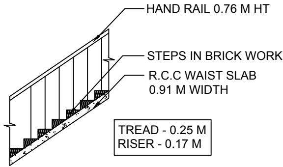
STEP DETAILS
