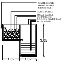
RECYCLING OF WASTE WATER FROM KITCHEN & BATHROOM
