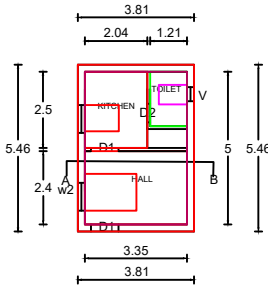
GROND FLOOR PLAN
