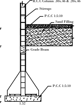
COLUMN DETAIL SCALE (1:50)
