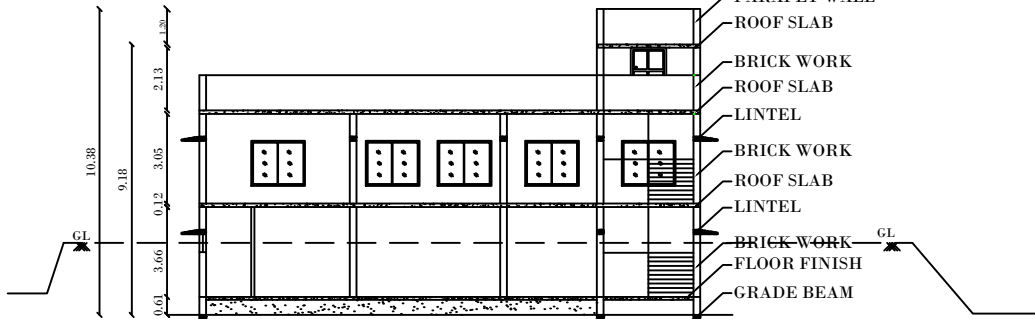
SHOP SECTION ON 'AB'
