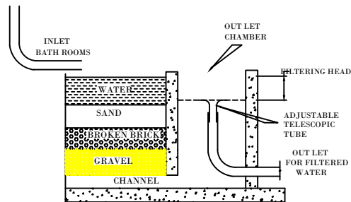
BATH WASTE WATER RECYCLE BED
