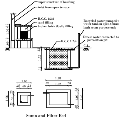
Sump and Filter Bed
