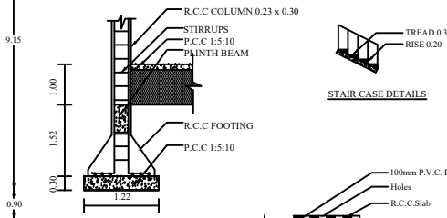
COLUMN DETAILS
