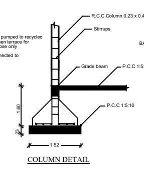
COLUMN DETAIL
