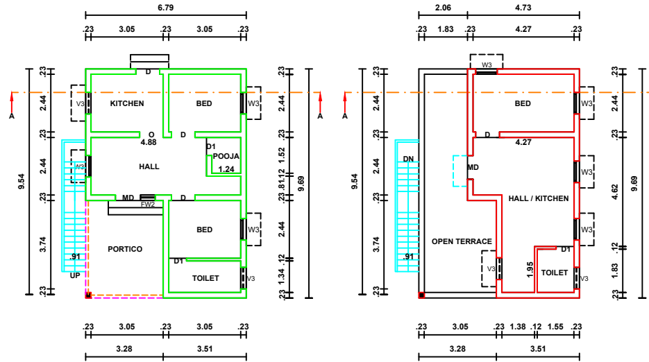
EXG.GROUND FLOOR PLAN
