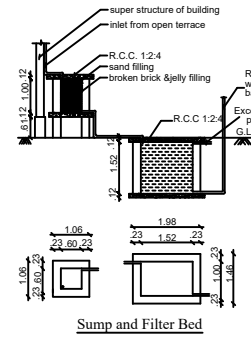
Sump and Filter Bed
