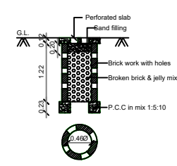
PERCOLATION PIT FOR 30 Sq. m. (Scale:- 1:50)
