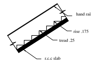
STAIR
