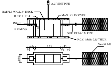
SEPTIC TANK AND TRENCH
