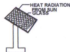
SOLAR SYSTEM
