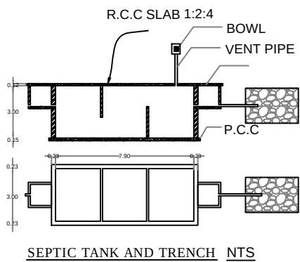
SEPTIC TANK AND TRENCH NTS
