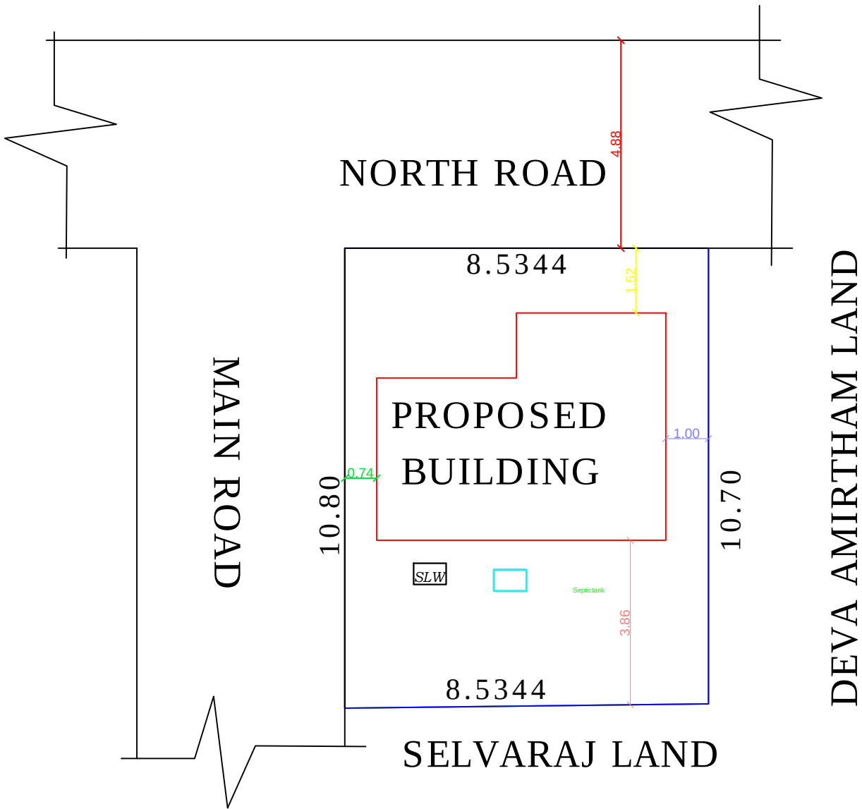
SITE PLAN
