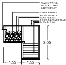
RECYCLING OF WASTE WATER FROM KITCHEN & BATHROOM
