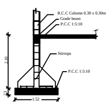
Column Detail
