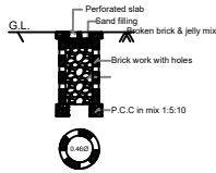
PERCOLATION PIT FOR 30 Sq.m (NOT FOR SCALE)
