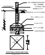
FOUNDATION DETAIL
