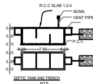
SEPTIC TANK AND TRENCH NTS
