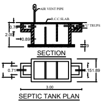
SECTION SEPTIC TANK PLAN
