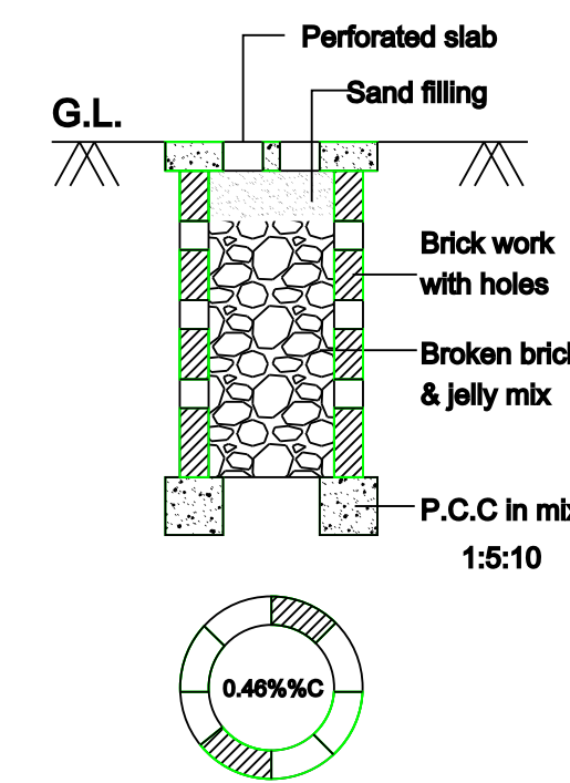
PERCOLATION PIT (NOT FOR SCALE)
