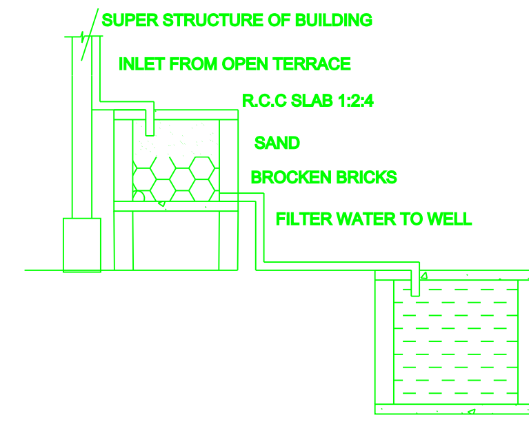
Rainwater harvesting
