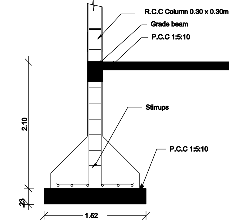
Column Detail
