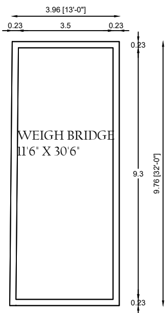
WEIGH BRIDGE PLAN
