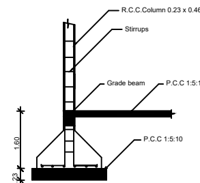
COLUMN DETAIL
