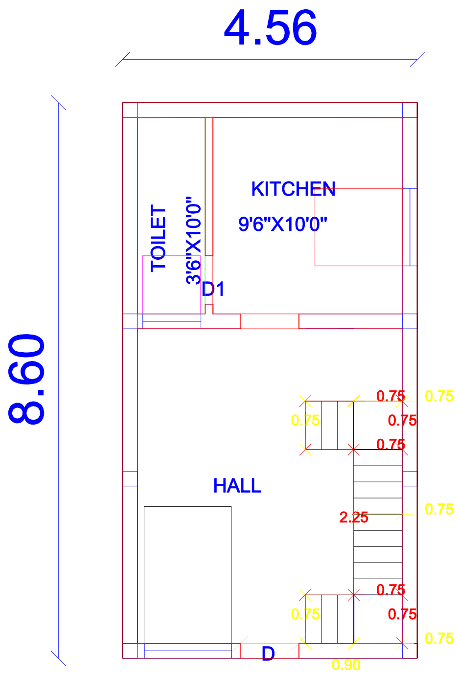
G.FLOOR PLAN
