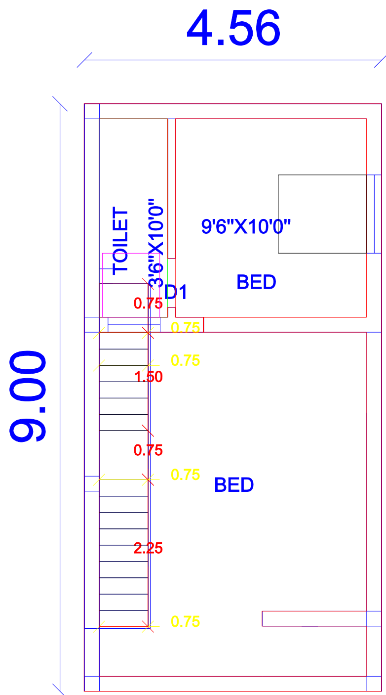
F.FLOOR PLAN
