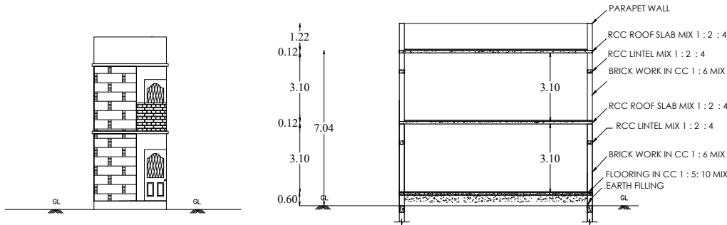
SECTION ON AB & ( HALF ELEVATION)
