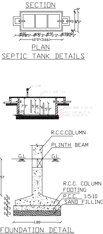
FOUNDATION DETAIL
