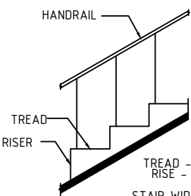
STAIRCASE DETAILS
