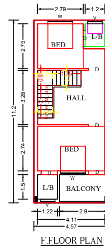
F.FLOOR PLAN
