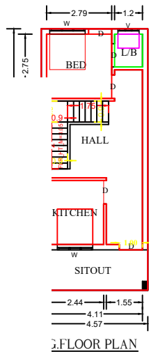
3.FLOOR PLAN
