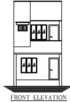
FRONT ELEVATION
