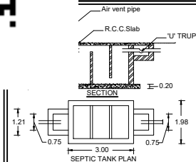
SEPTIC TANK PLAN
