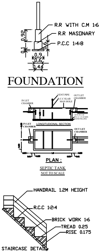
STAIRCASE DETAILS
