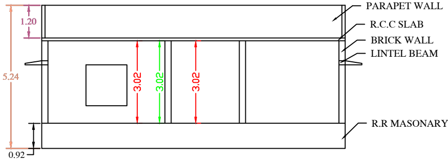
SECTION AT X-X'
