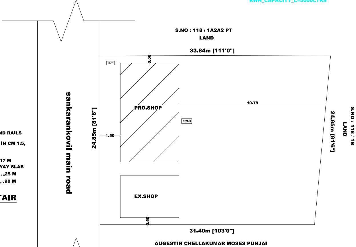
SITE PLAN
