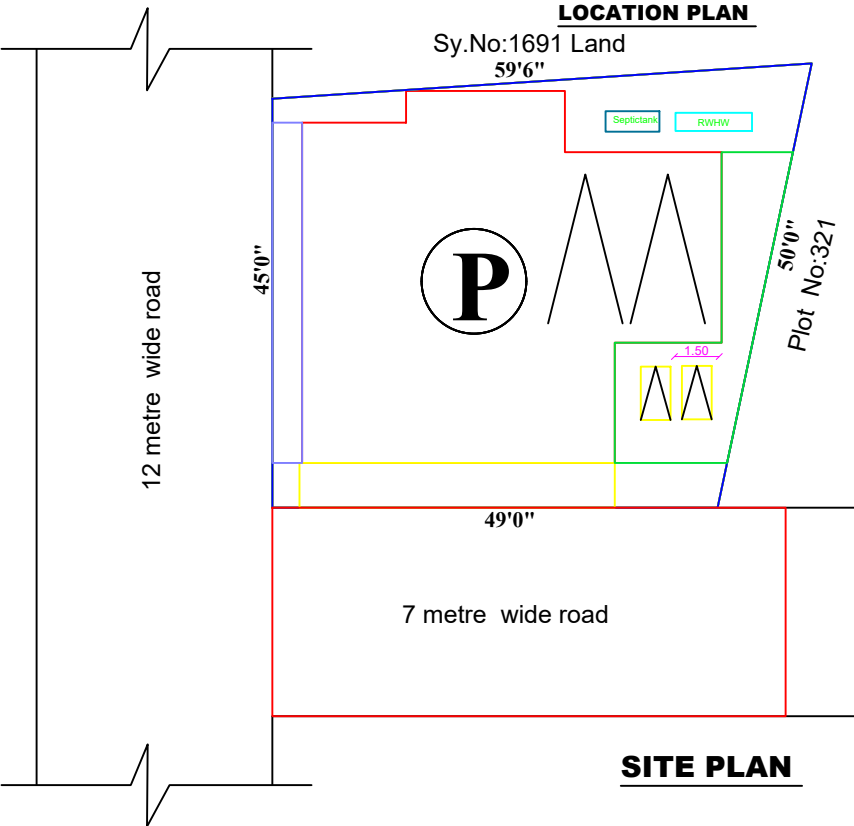
LOCATION PLAN
