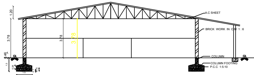
BRICK KILN SECTION ON 'AA'
