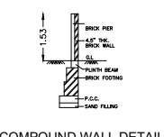
COMPOUND WALL DETAIL
