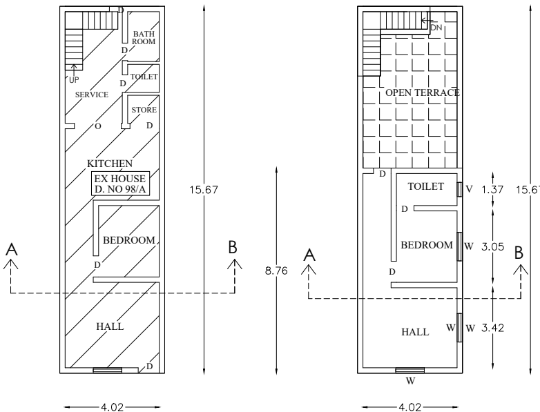
EX GROUND FLOOR PLAN
