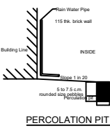
PERCOLATION PIT
