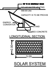
SOLAR SYSTEM
