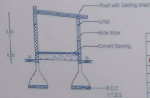
CROSS SECTION ON 'AB'
