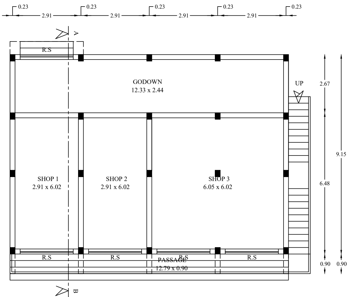
PLAN(APPROVED)
