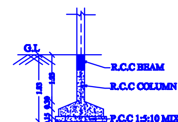
SECTION OF FOOTING
