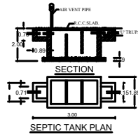
SEPTIC TANK PLAN
