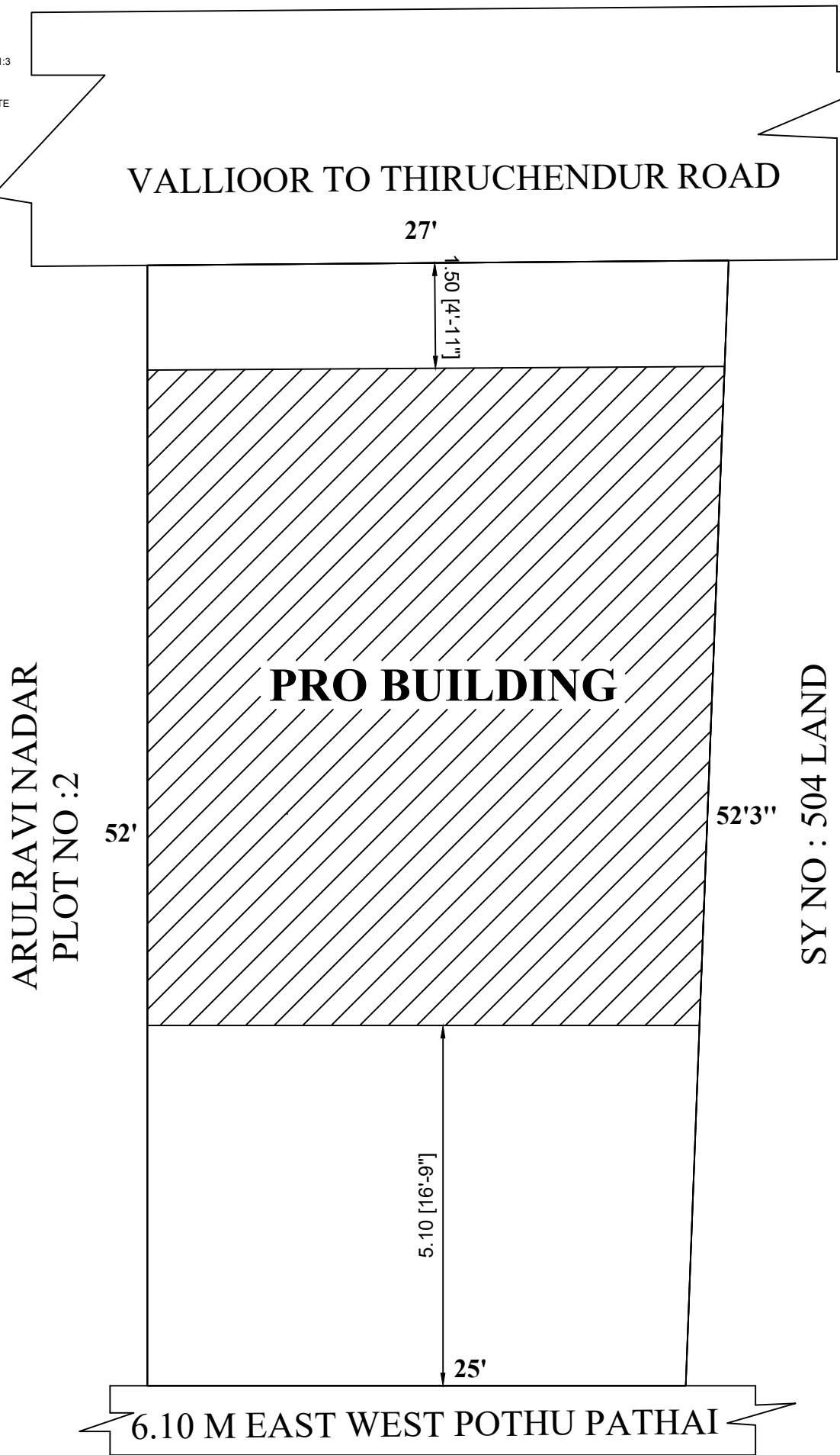
SITE PLAN
