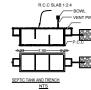
SEPTIC TANK AND TRENCH NTS
