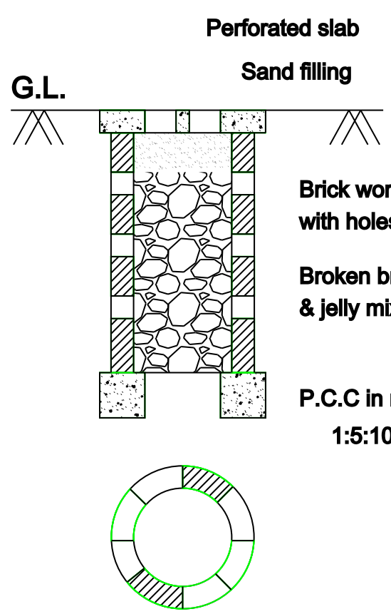
PERCOLATION PIT (NOT FOR SCALE)
