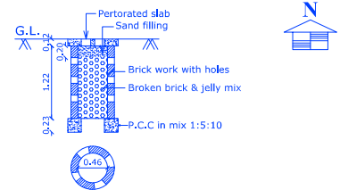
PERCOLATION PIT FOR 30 Sq. m. (Scale:- 1:50)
