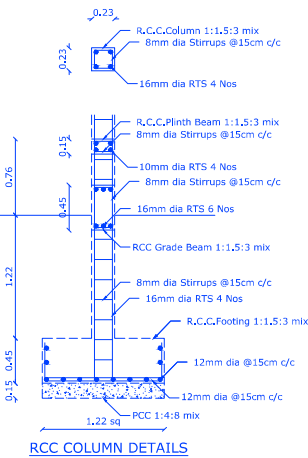
RCC COLUMN DETAILS
