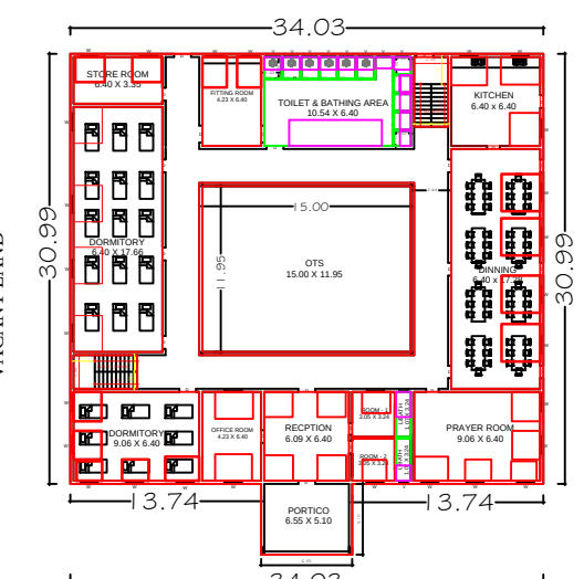
SCALE: NTS.
